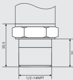
1/2-14NPT
