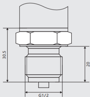
G1/2
