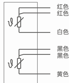
2 x Pt100
