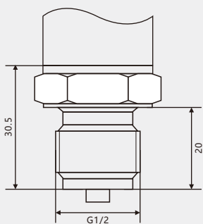
G1/2
