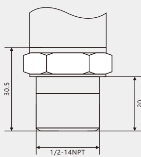
1/2-14NPT
